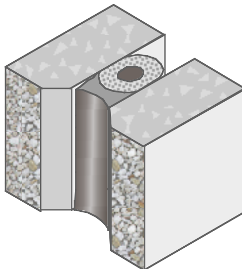
Figur 1. Adhesionsbrott
